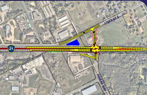
CONCEPT LAYOUT
